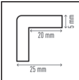
Corner protection profile C20 #1101-130 - adhesive #1111-130 - magnetic
