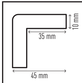
Corner protection profile C35 #1102-130 - adhesive #1112-130 - magnetic
