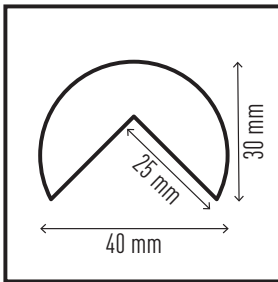
Corner protection profile C25R #1100-130 - adhesive #1110-130 - magnetic
