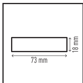
Surface protection profile S18 #1108-130
