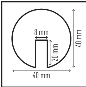
Edge protection profile E8R #1126-130
