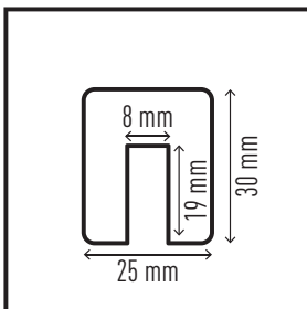
Edge protection profile E8 #1127-130
