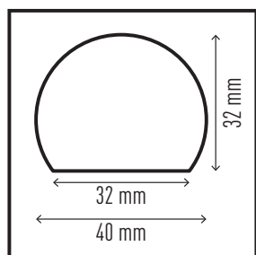
Surface protection profile S32R #1109-130
