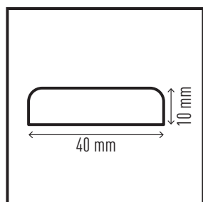
Surface protection profile S10 #1107-130
