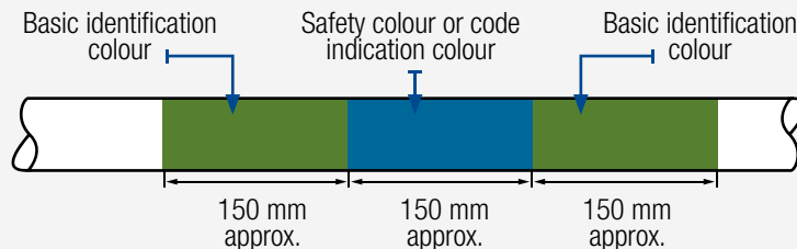
Example for >100 mm pipe diameter
